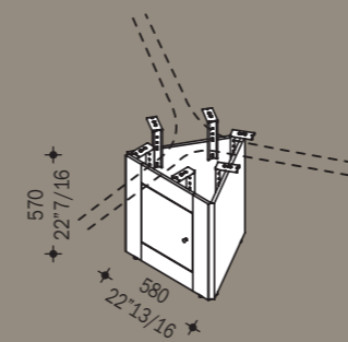
P5519T Basamento triangolare 120° Base for cluster solution 120° Base triangulaire 120° Columna central para banch 120°
