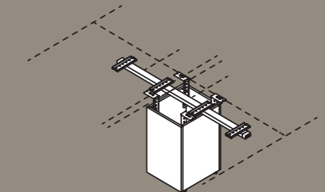
P5519MT Basamento bench doppio Bases for bench solution Base de support Columna central para banch doble
