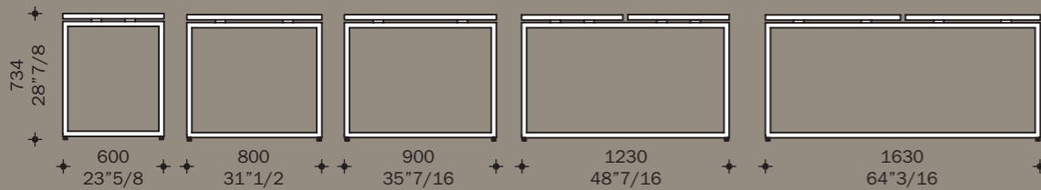
P5519A2 Gamba ad anello regolabile / Adjustable closed loop leg / Pied fermè réglable en ht. / Pata anillo regulable en altura
