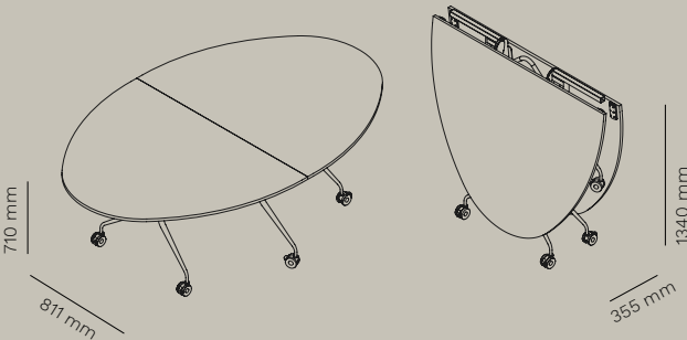
ARGO LIBRO 286T Round / 286T Elliptical
