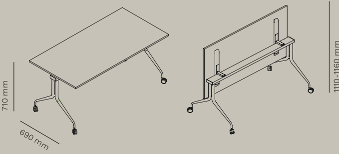
ARGO TILTING 206R
