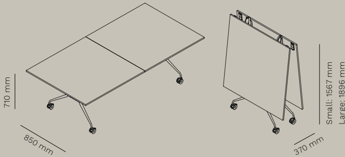
ARGO LIBRO XL 286XL Small / 286XL Large
